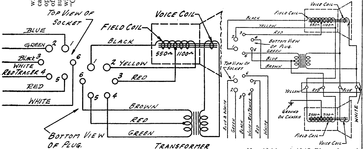
No. 4245 Electrodynamic Speaker and Connections
